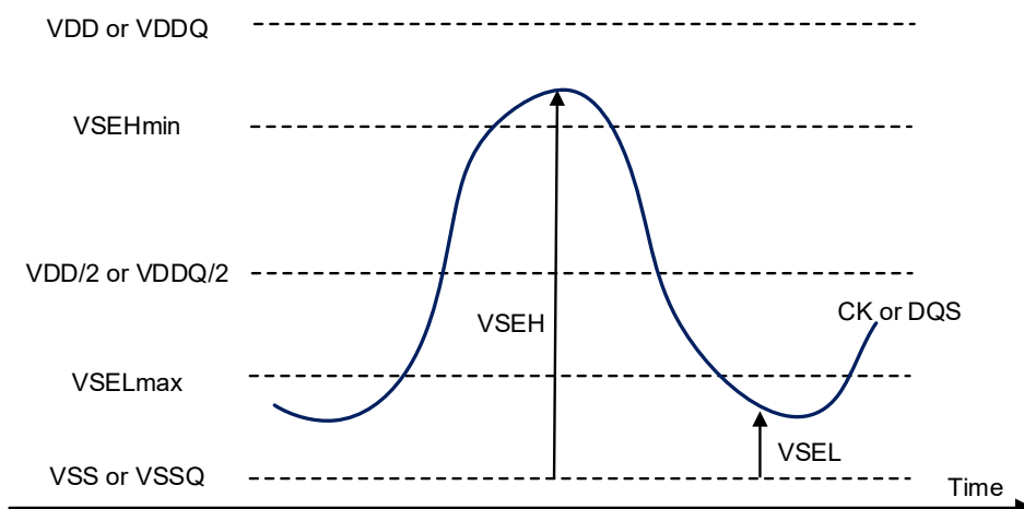
Figure 5-3. Single-ended Requirement for Differential Signals.
