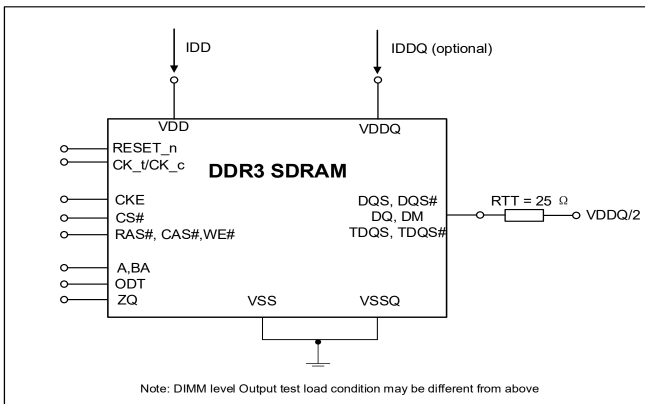
Figure 7-1. Measurement Setup and Test Load for IDD and IDDQ (optional) Measurements
