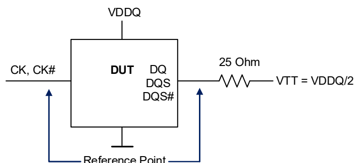
Figure 6-3. Reference Load for AC Timing and Output Slew Rate
