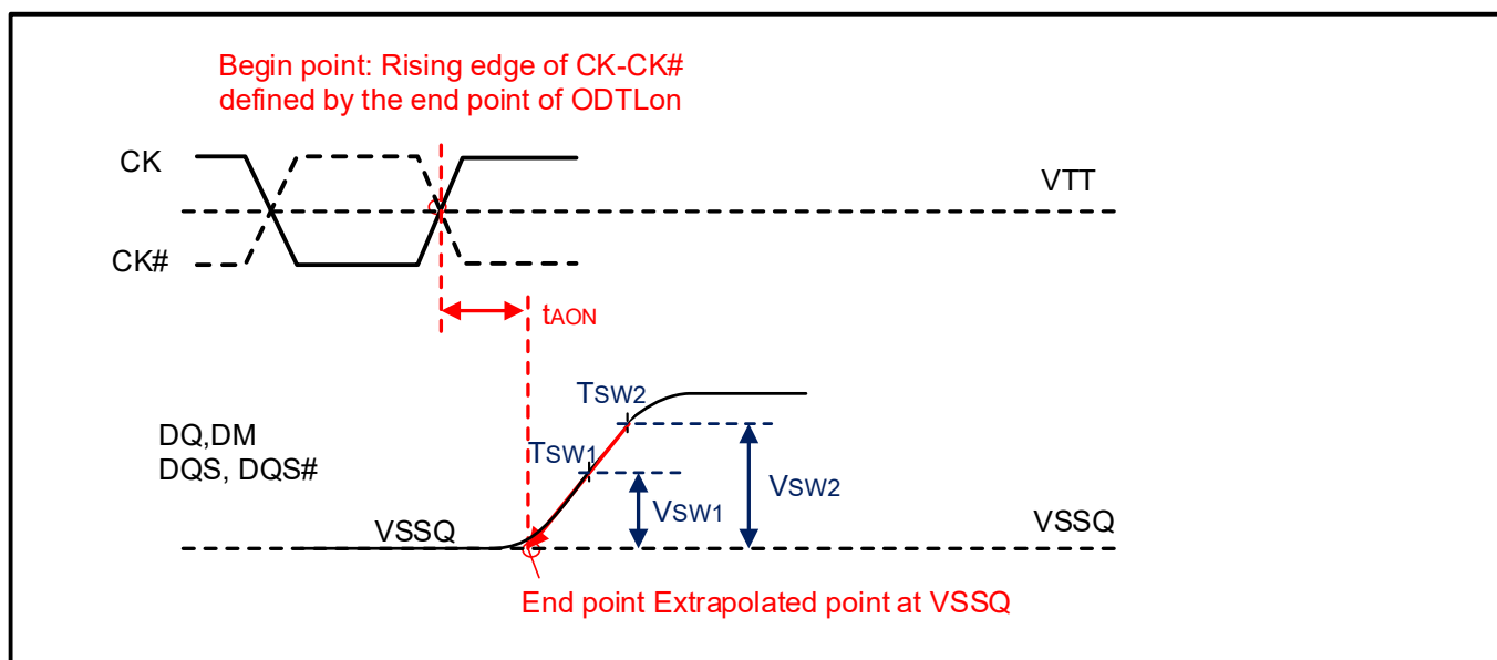
Figure 6-9. Definition of t_{AON}
