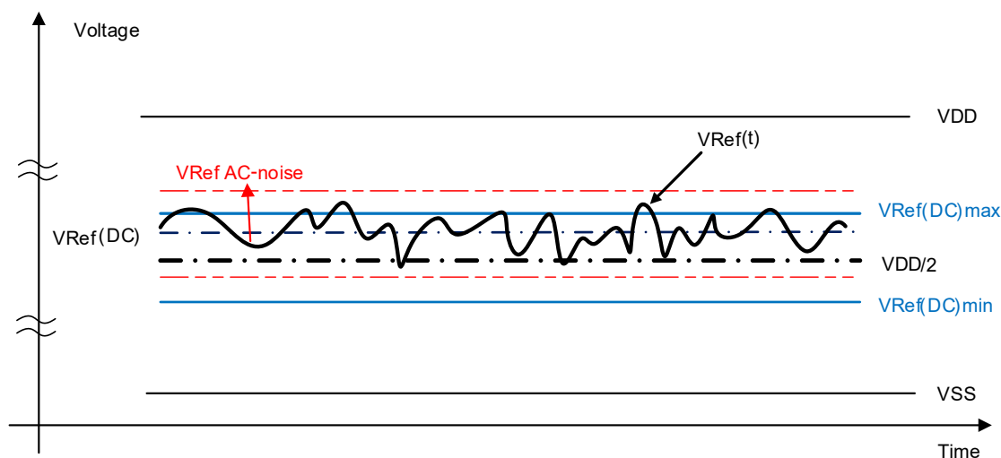
Figure 5-1. Illustration of V_{Ref}(DC) tolerance and V_{Ref} ac-noise limits
