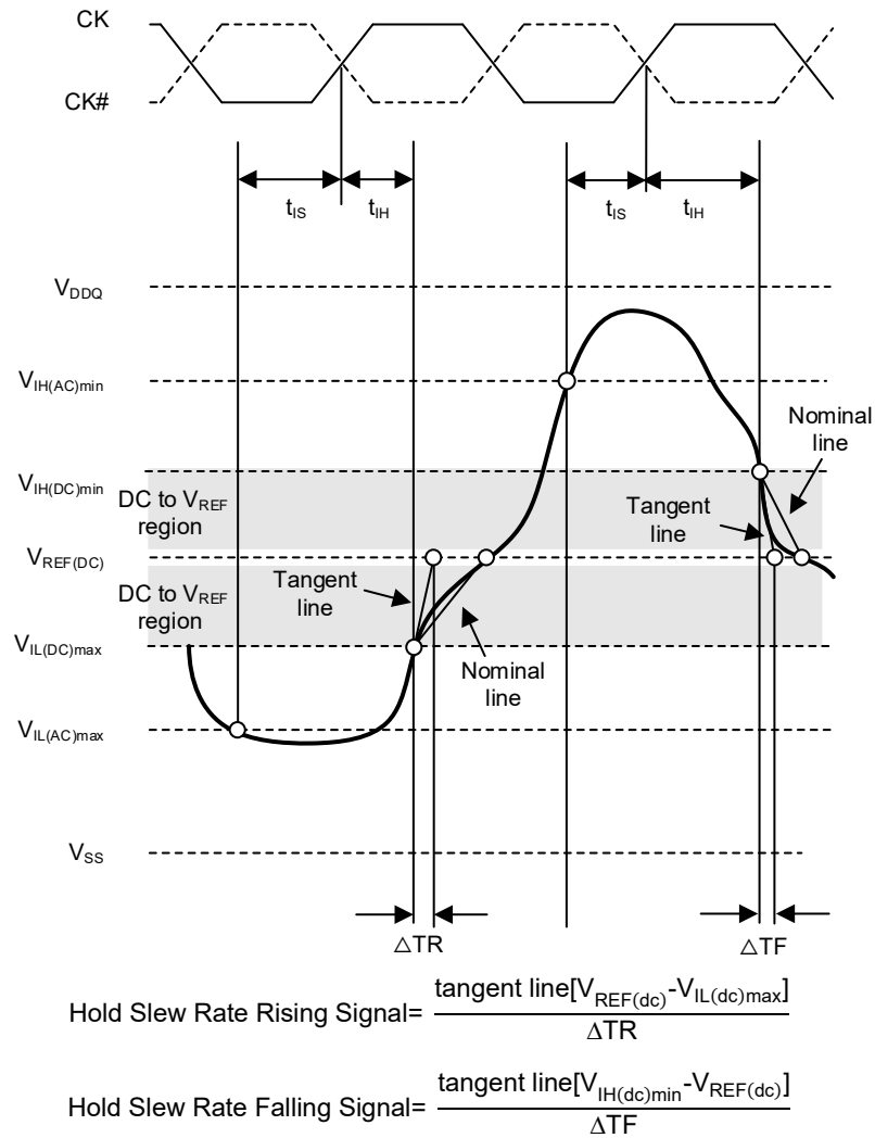
Figure 12-4. Illustration of tangent line for hold time t_H (for ADD/CMD with respect to clock)
