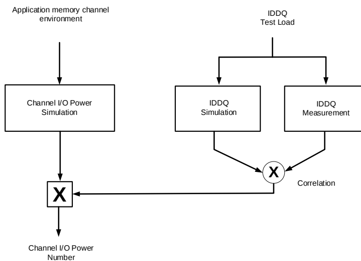
Figure 9-2. Correlation from Simulated Channel I/O Power to Actual Channel I/O Power Supported by IDDQ Measurement
