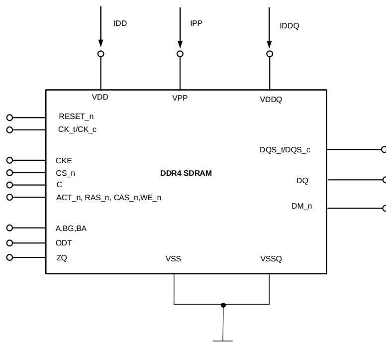
Figure 9-1. Measurement Setup and Test Load for IDD, IPP and IDDQ Measurements
