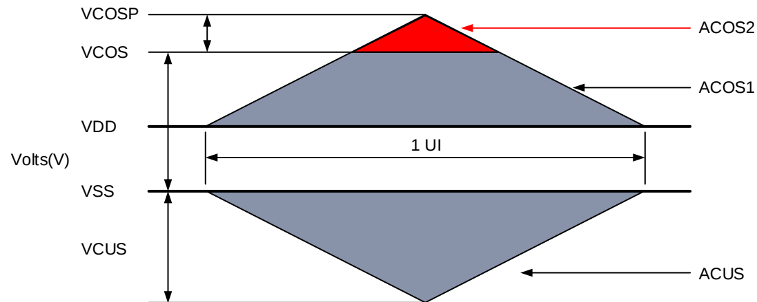
Figure 6-5. Clock Overshoot and Undershoot Definition
