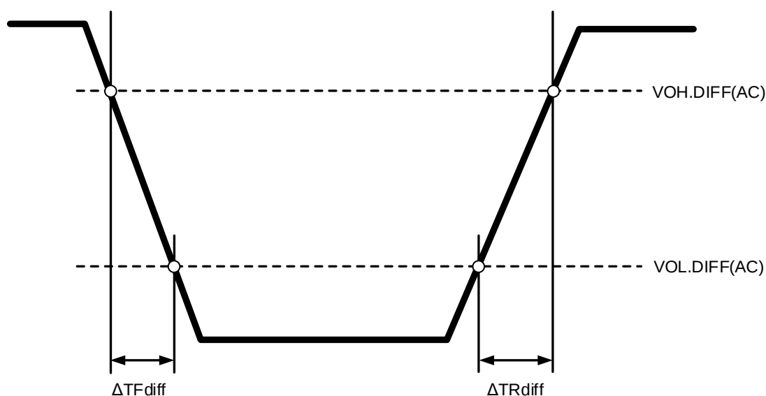
Figure 7-5. Differential Output Slew Rate Definition
