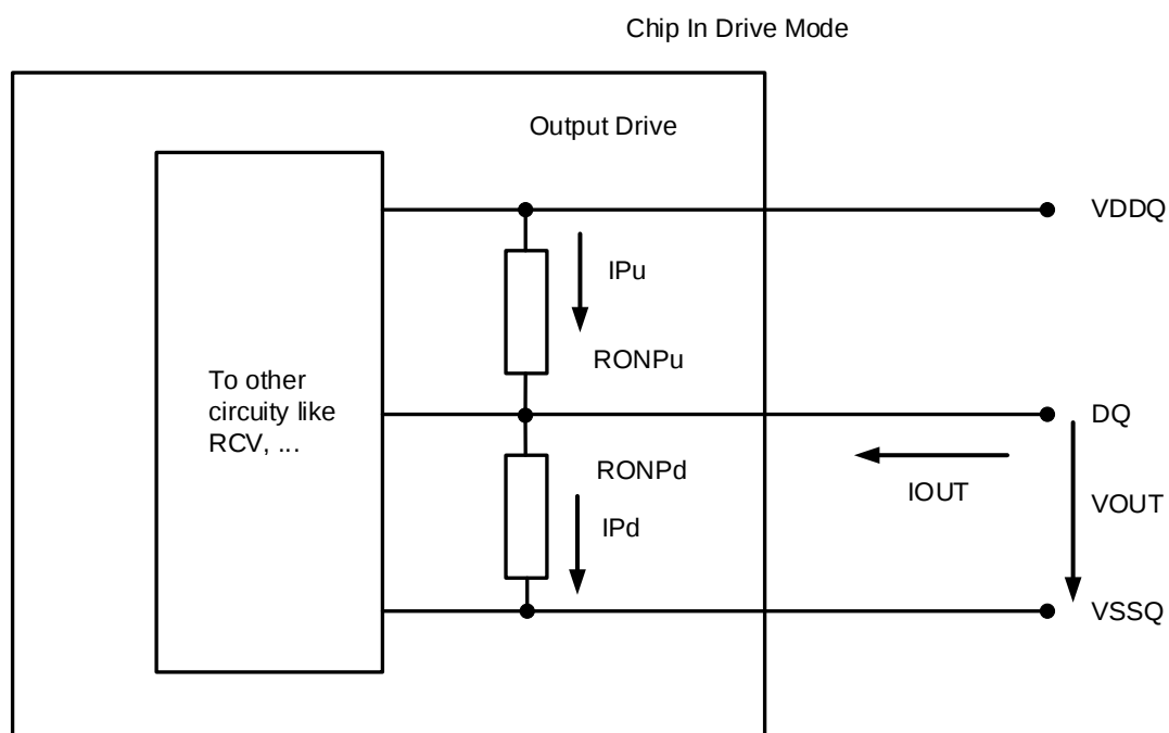
Figure 7-1. Output Driver
