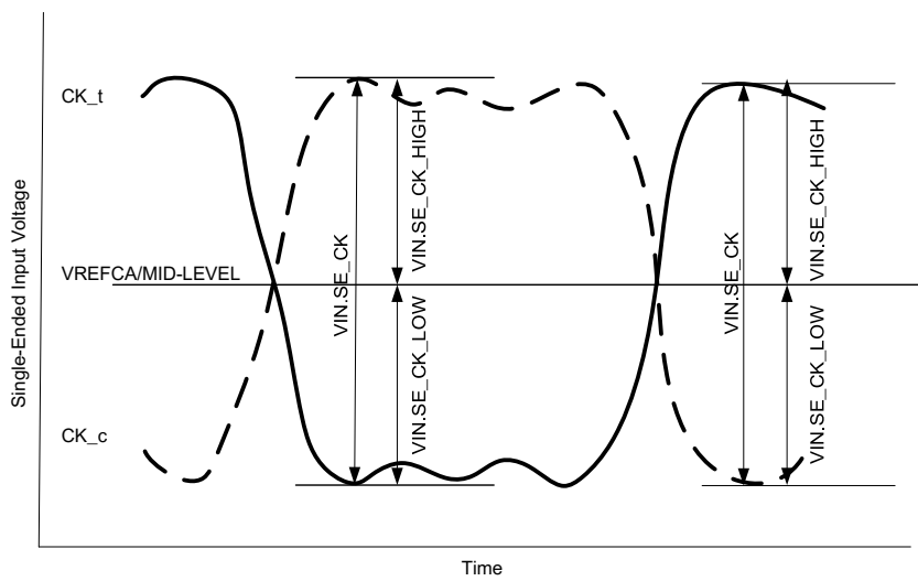
Figure 7-6 Clock Single-Ended Input Voltage
