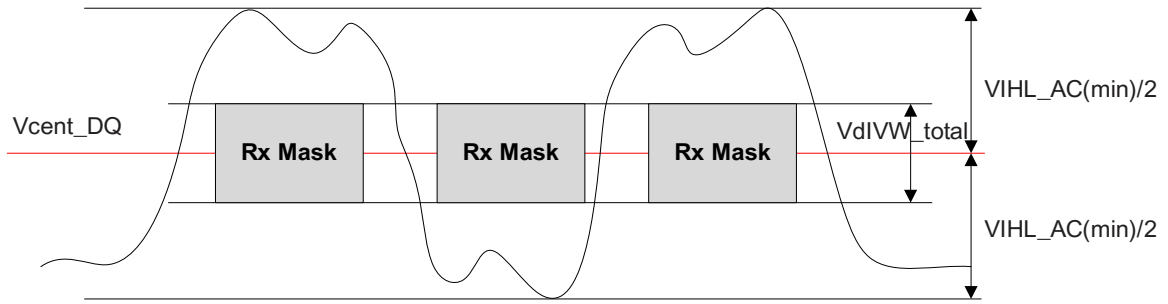
Figure 11-12 DQ VIHL_AC definition (for Each Input Pulse)
