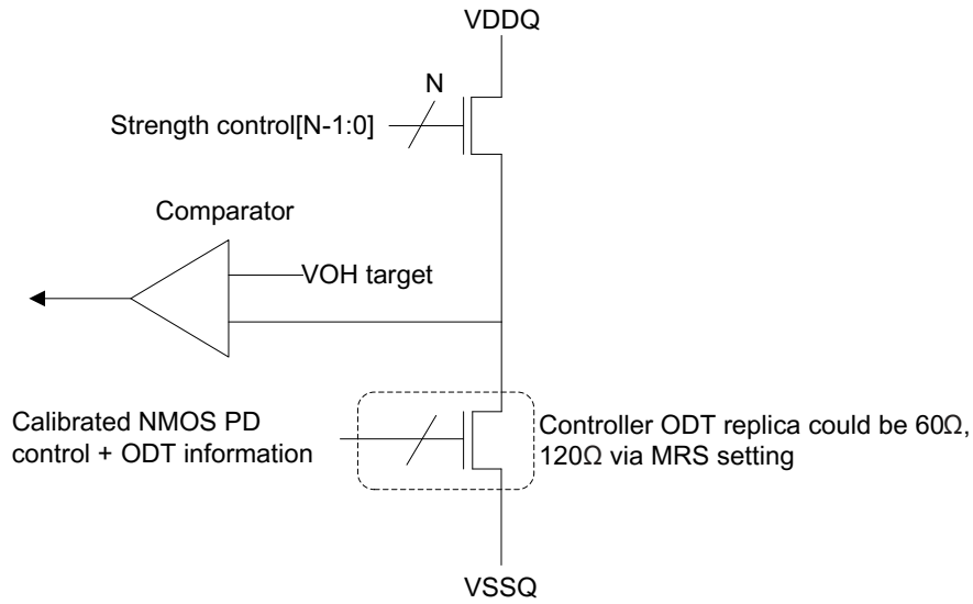
Figure 8-7 Pull-Up Calibration
