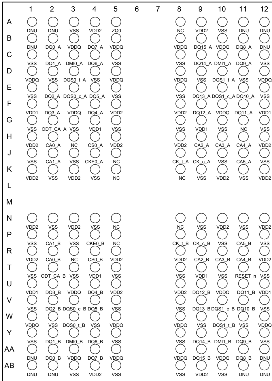
Figure 2-3 200-Ball Dual-Channel, Single-Rank Discrete FBGA (2GB x32 I/O)
