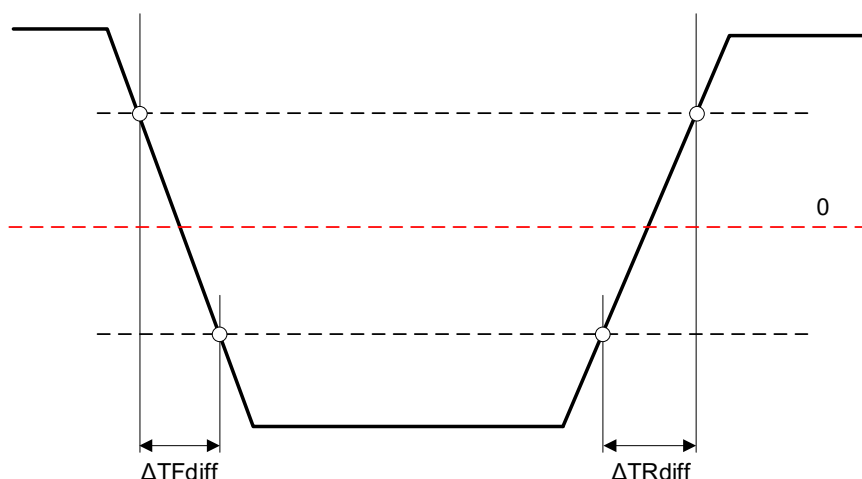
Figure 8-2 Differential Output Slew Rate Definition
