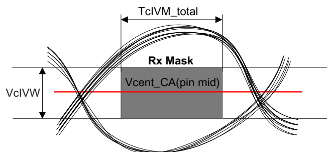
Figure 11-1 CA Receiver(Rx) Mask
