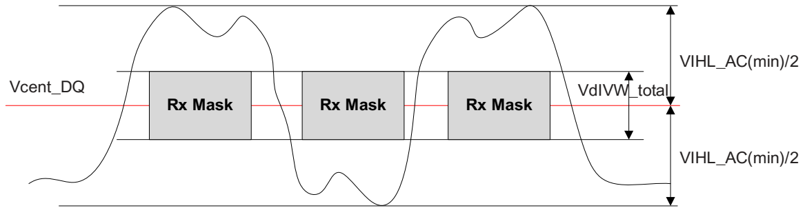
Figure 11-12 DQ VIHL\_LAC definition (for Each Input Pulse)
