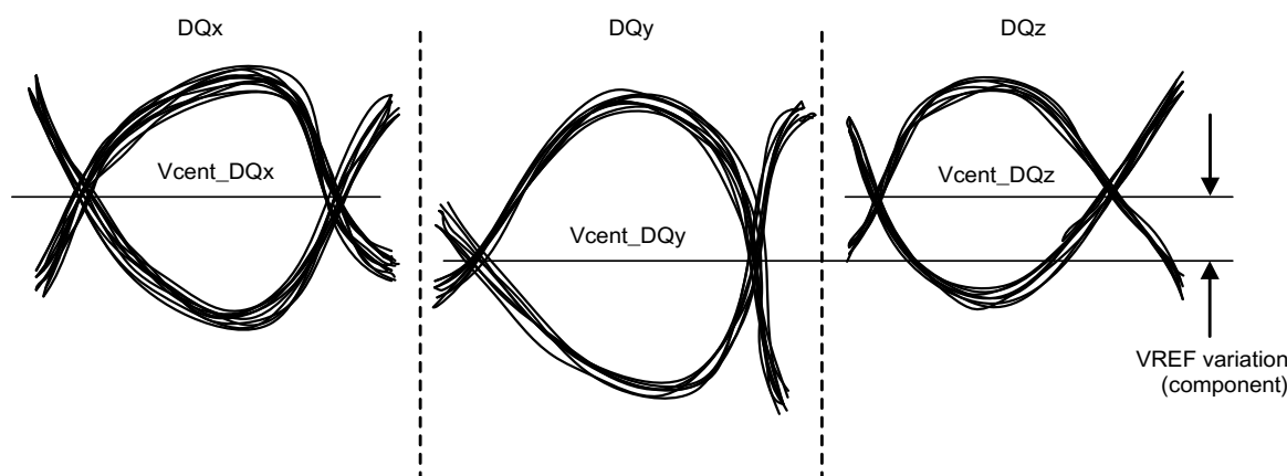
Figure 11-9 Across Pin VREF DQ Voltage Variation
