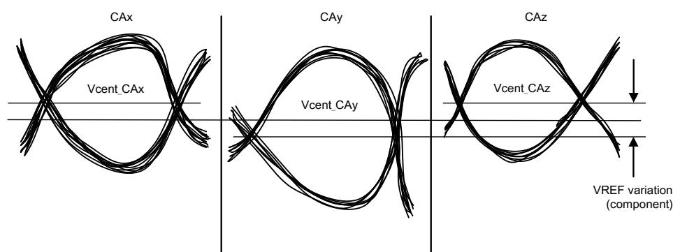
Figure 11-2 Across Pin VREFCA Voltage Variation
