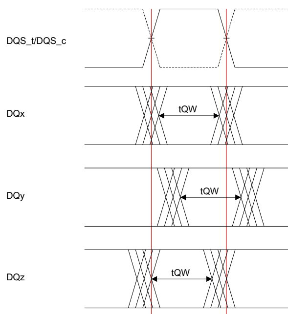
Figure 11-7 Read Data Timing tQW Valid Window Defined per DQ Signal
