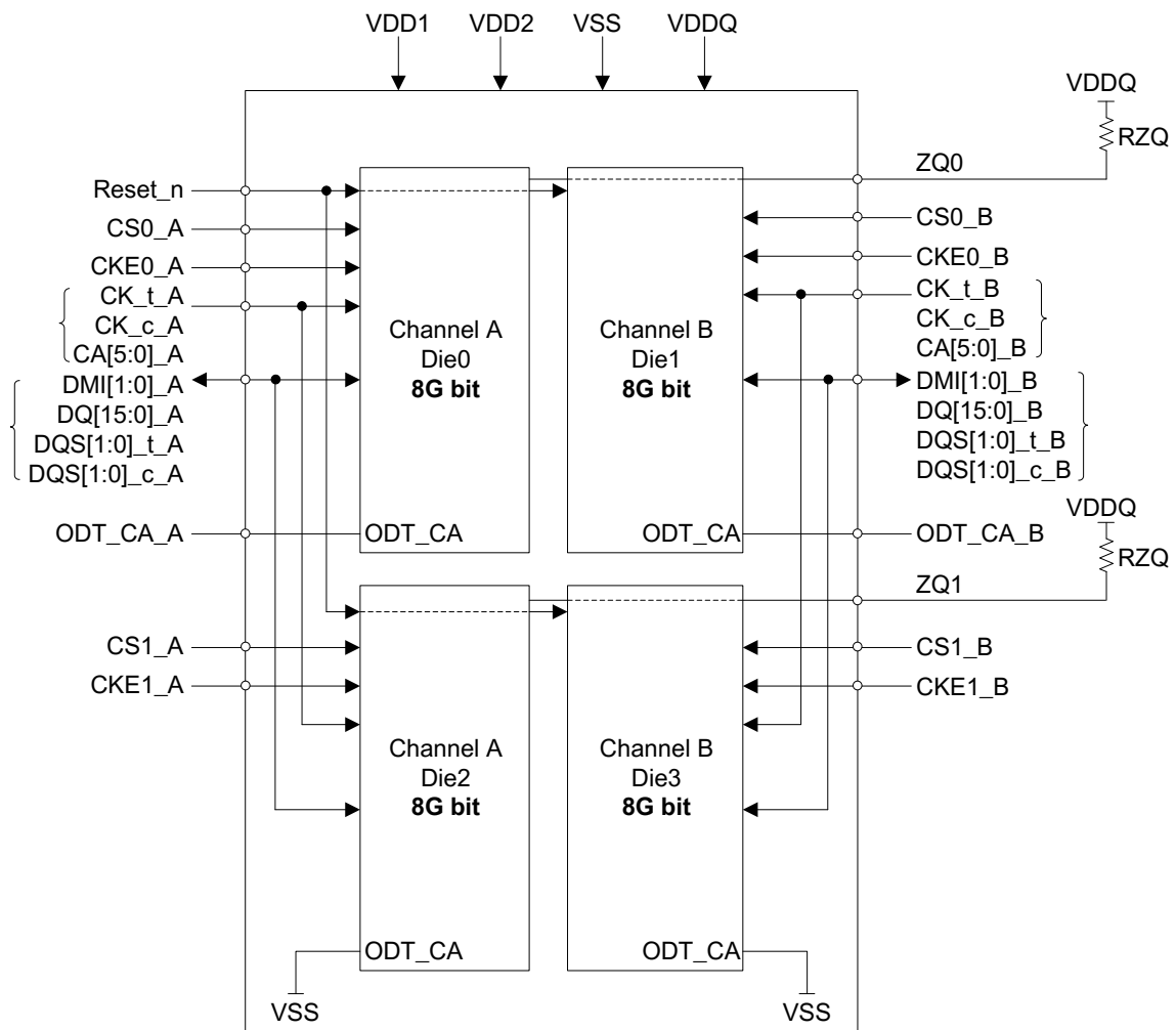
Figure 2-8 Quad-Die, Dual-Channel, Dual-Rank Package Block Diagram (4GB x32 I/O)
