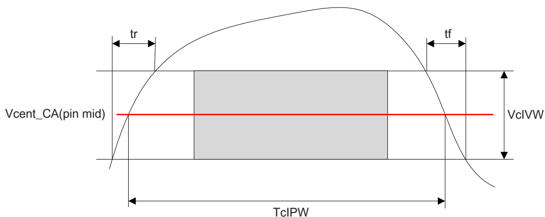
Figure 11-4 CA TcIPW and SRIN_cIVW definition (for each input pulse)
