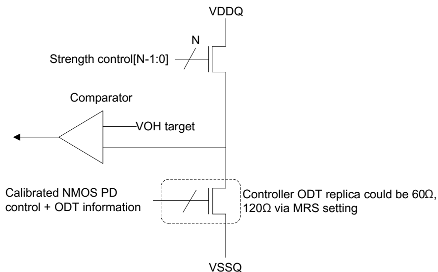
Figure 8-7 Pull-Up Calibration
