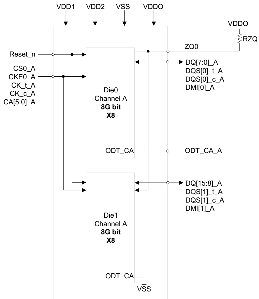
Figure 2-6 Dual-Die, Single-Channel, Single-Rank Package Block Diagram (2GB x16 I/O)
