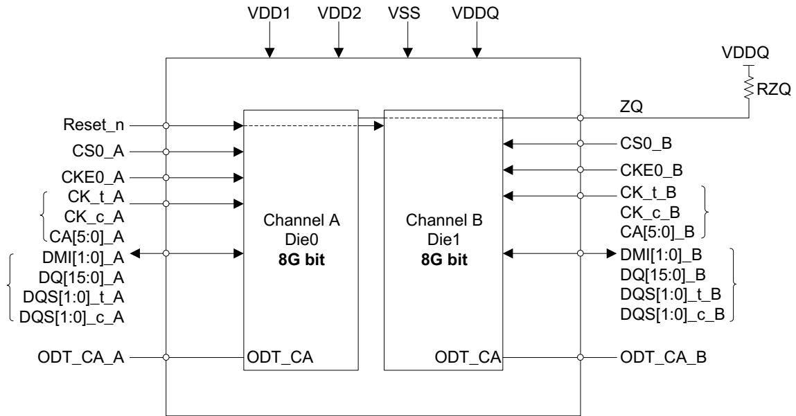
Figure 2-7 Dual-Die, Dual-Channel, Single-Rank Package Block Diagram (2GB x32 I/O)
