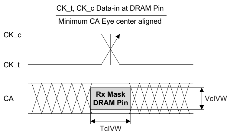
Figure 11-3 CA Timings at the DRAM Pins
