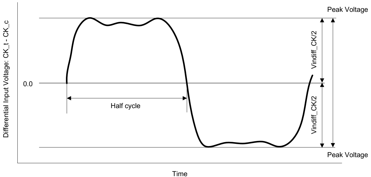
Figure 7-4 CK Differential Input Voltage
