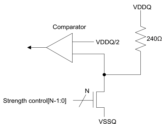
Figure 8-6 Pull-Down Calibration
