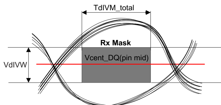
Figure 11-8 DQ Receiver(Rx) Mask
