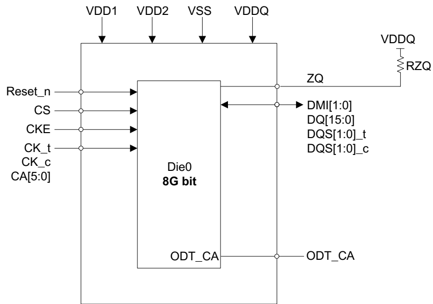
Figure 2-5 Single-Die, Single-Channel, Single-Rank Package Block Diagram (1GB x16 I/O)
