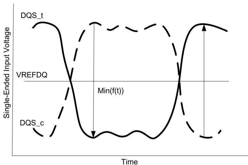
Figure 7-10 Definition of Differential DQS Peak Voltage
