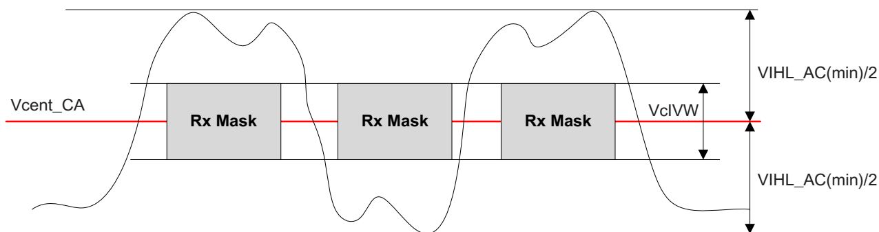
Figure 11-5 CA VIH_L_AC Definition (for Each Input Pulse)
