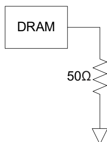
Figure 8-4 Driver Output Reference Load for Timing and Slew Rate
